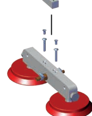
Vacuum modular unit MST-0541-10-02-00-0
