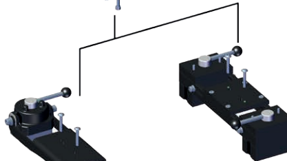
Magnetic spacing-adjustable unit ZSP-0523-19-00-00-0
